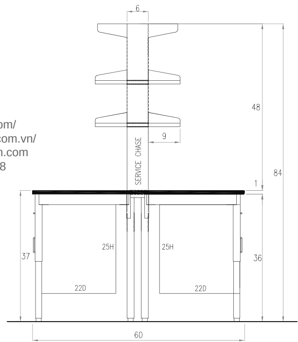
End View
